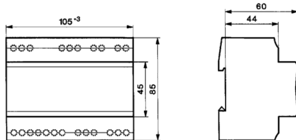
Dimensional details
