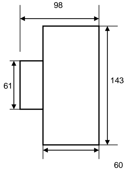
NH0184SQ 2 X 35W IP20 GU10 Wall Mounted Fitting
