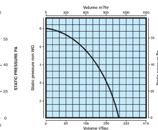
Performance Graph XFS300 Series 1100m 3 /hr, 306 litres per second
