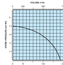
Performance Graph XFS230 Series 668m 3 /hr, 185 litres per second
