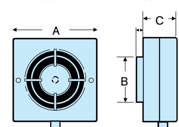
Dimensions XF120MH Series
