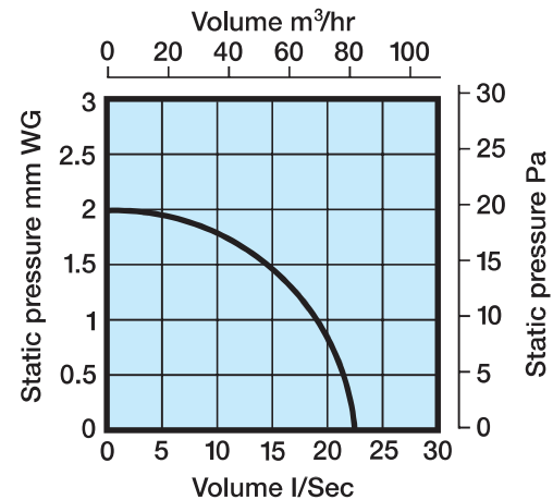
Performance Graph XF/WF100 Series 85m 3 /hr, 23 l/s
